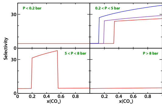
Figure 2. Curves of selectivity as a function of CO 2 composition of the mixture, for different fixed values of the total pressure (0.1, 0.5, 1, 4, 7, and 10 bar), in MIL-53 (Al) at 304 K.
