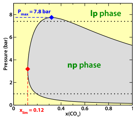
Figure 1. Predicted diagram of stability of the np and lp phases of MIL-53 (Al) upon adsorption of a CO 2 /CH 4 mixture at 304 K, as a function of total pressure and mixture composition. The horizontal dotted lines correspond to the constant-pressure experiments. 7
