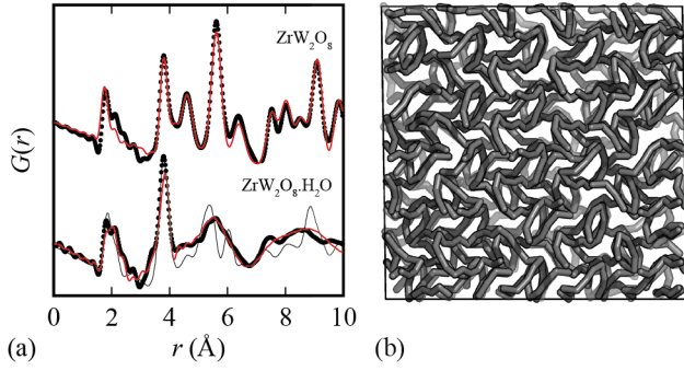
FIG. 3. (a) X-ray PDFs G(r) of anhydrous (top) and hydrated (bottom) \text{ZrW}_2\text{O}_8 : data as points and fits as lines. For \text{ZrW}_2\text{O}_8 a satisfactory fit is obtained using the model of Ref. [3] (red lines). For the hydrate, the DFT P2_12_12_1 model fits at low r but cannot reproduce the broad oscillations at r > 4 \text{ \AA} (thin black line). Instead, the PDF calculated from our disordered spaghetti model (red line) captures all features. (b) The relaxed GULP model for a \text{ZrW}_2\text{O}_8 \cdot \text{H}_2\text{O} spaghetti configuration as described in the text: only W—O—W linkages are shown, using grey cylinders [cf. Fig. 2(d)].
